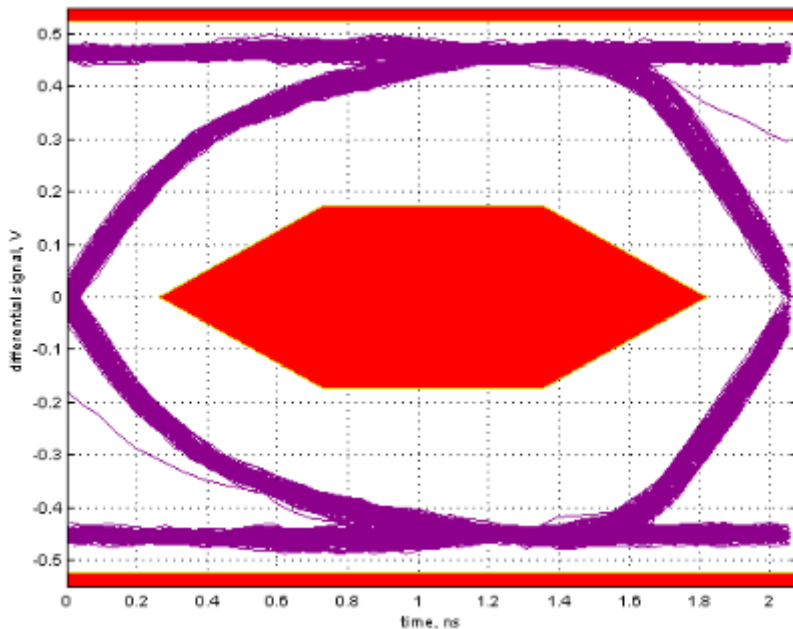
图 1-8 USB 2.0 High-speed Far End SQ Eye Diagram
